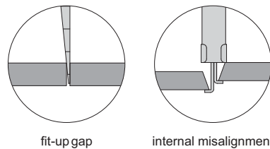
fit-up gap
