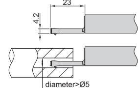
small hole probe (optional), code ISR-C002-PROBE
