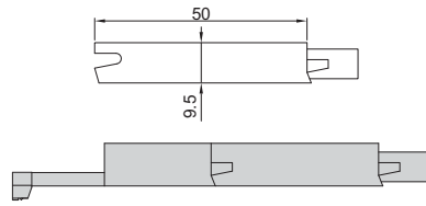
extension rod (optional), code ISR-C002-ER
