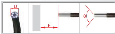
lens with LED focus distance angle of view
