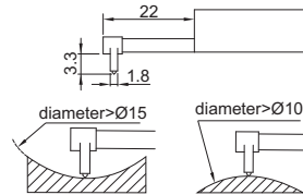
curved surface probe (optional), code ISR-C002-SUR
