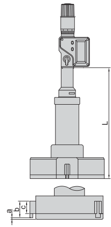
Type D 50-300mm, carbide measuring points
