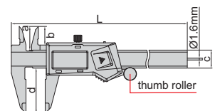
round depth bar Ø1.6mm
