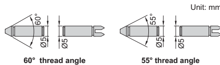
60° thread angle
