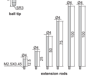
extension rods
