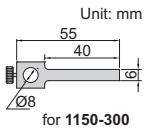
dial test indicator holder (included)
