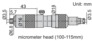
micrometer head (100-115mm)
