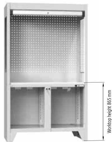
Control workstation body, width 1200 mm 27 x 27D
