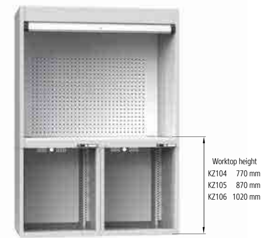
Control workstation body, width 1462 mm 36 x 36D
